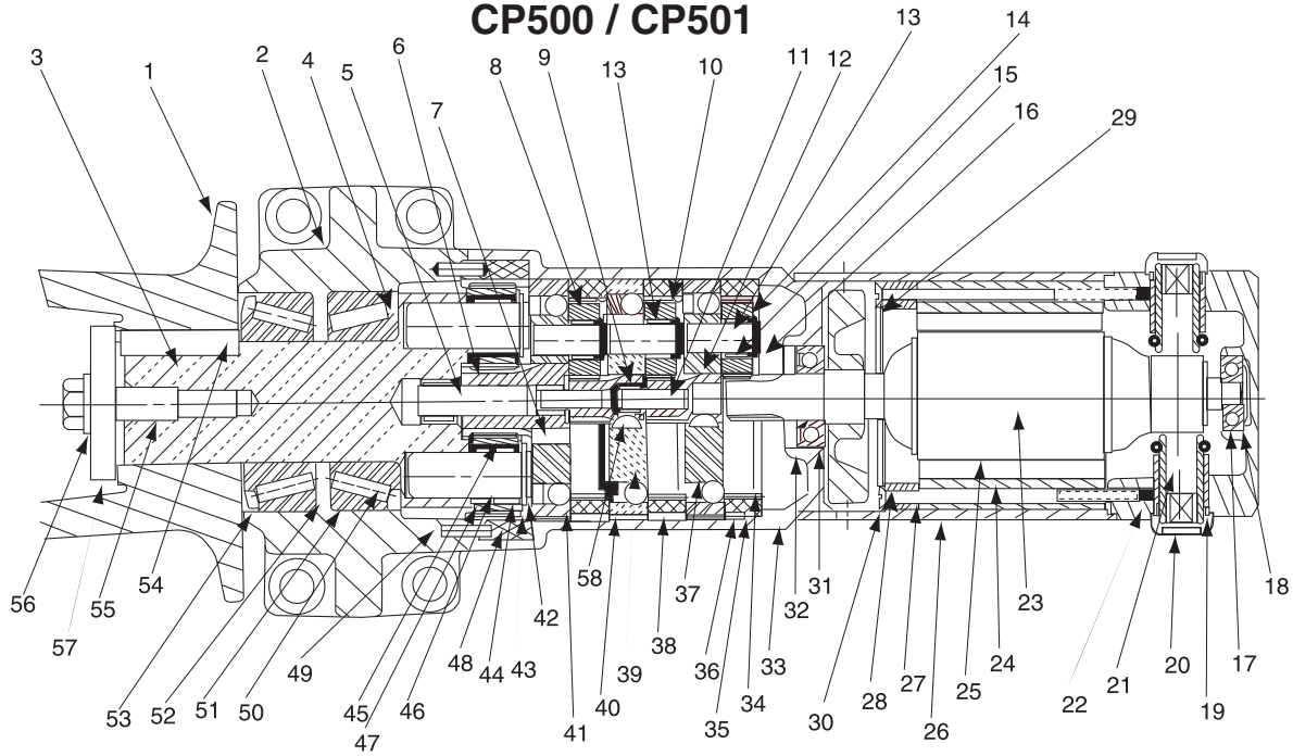
Parts List Motor and Capstan Assembly
