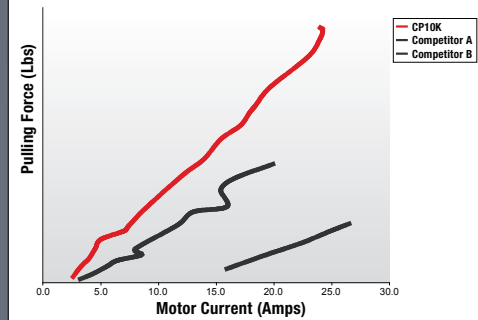
LOAD CELL READING VS. MOTOR CURRENT
